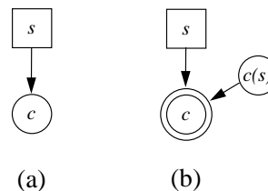
Figure 5: A transformation to Howard Canonical Form.
