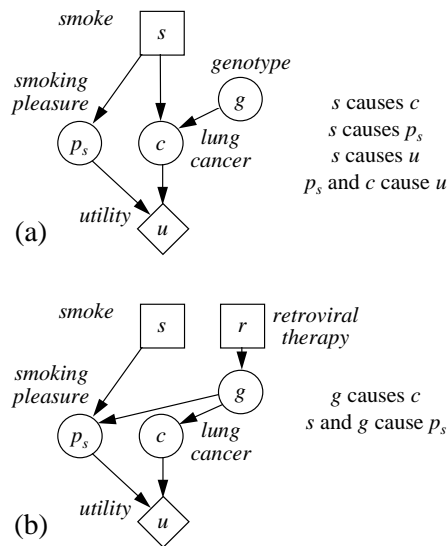
Figure 2: Variants the decision problem in Figure 1.
