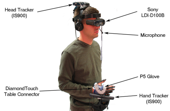
Figure 5. User's AR interaction devices.
