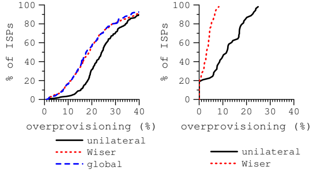
Figure 4: Wiser reduces overprovisioning level. Left: Pairs of ISPs. Right: The entire internetwork topology.
