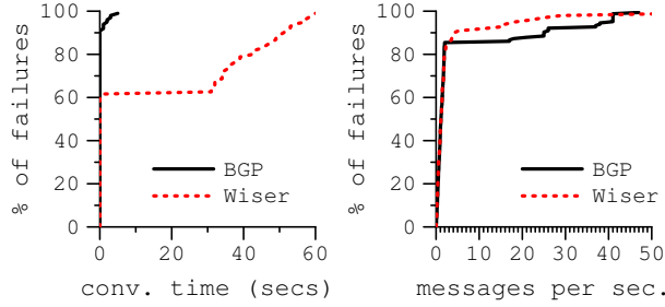
Figure 6: The convergence time and routing message overhead of Wiser. Left: The CDF of convergence time. Right: The CDF of maximum rate of routing messages.
