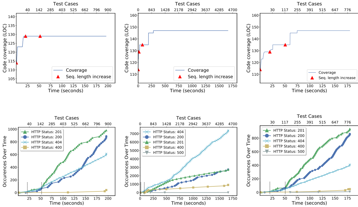
Fig. 5: Code Coverage and HTTP Status Codes Over Time. Shows the increase in code coverage over time (top) and the cumulative number of HTTP status codes received over time (bottom), for the simple blog posts service. Left: REST-ler ignores dependencies among request types. Center: REST-ler ignores dynamic feedback. Right: REST-ler utilizes both dependencies among request types and dynamic feedback. When leveraging both techniques, REST-ler achieves the best code coverage and finds the planted 500 “Internal Server Error” bug with the least number of tests.
