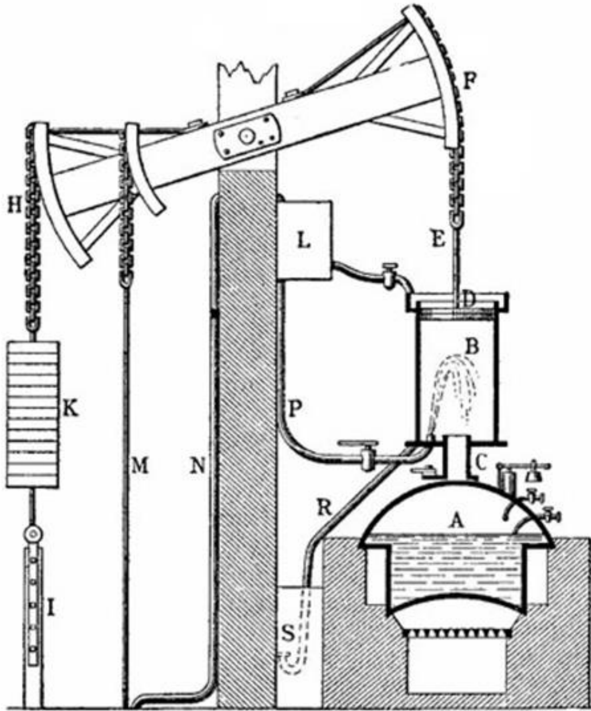
Thomas Newcomen, 1712
