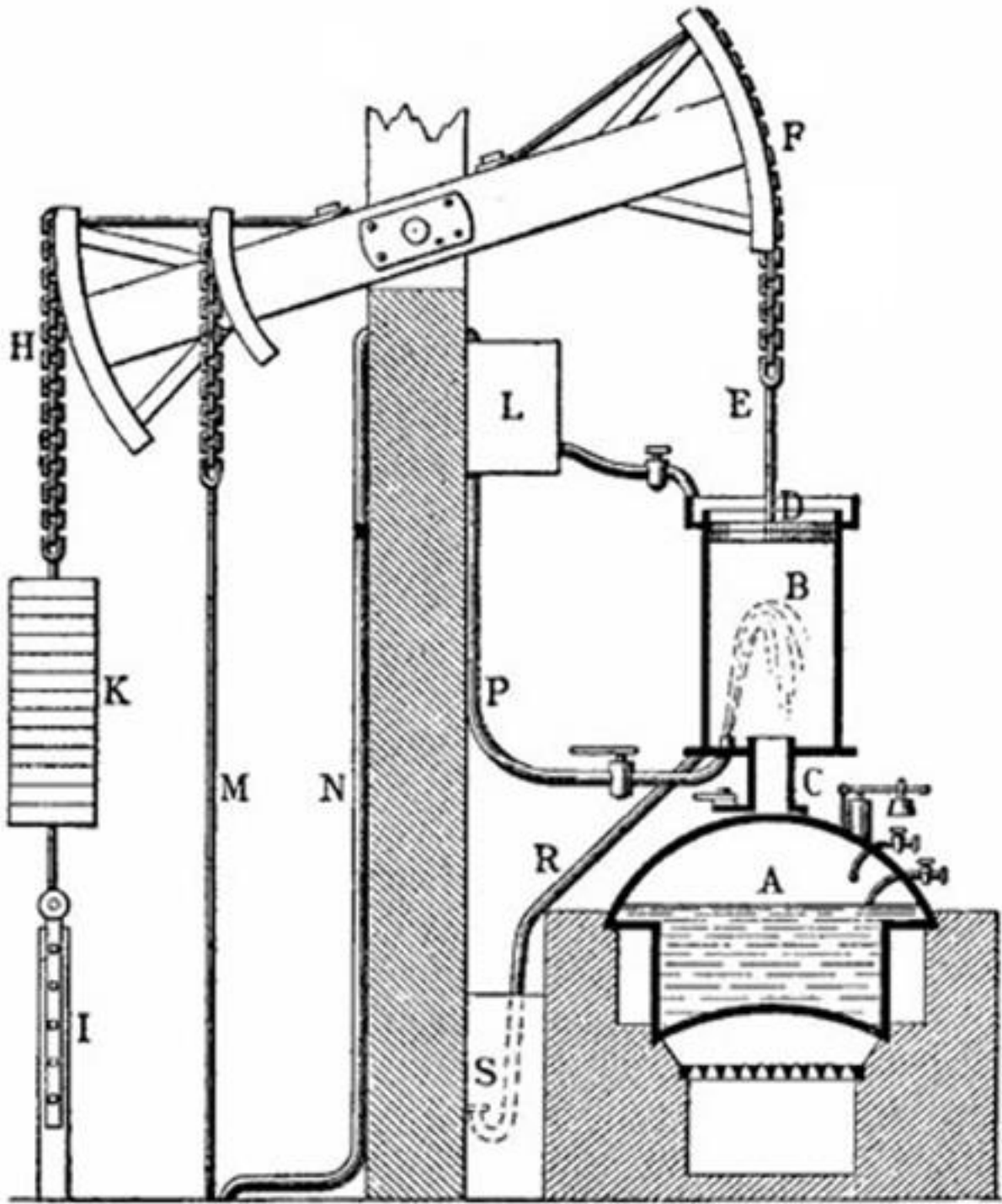
Thomas Newcomen, 1712
