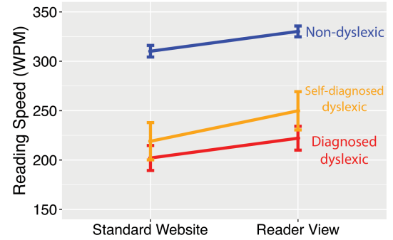
Figure 2: Average reading speed across non-dyslexic, diagnosed dyslexic, and self-diagnosed dyslexic participants in Words per Minute for Standard Webpages and their Reader Views. Error bars show standard error.
