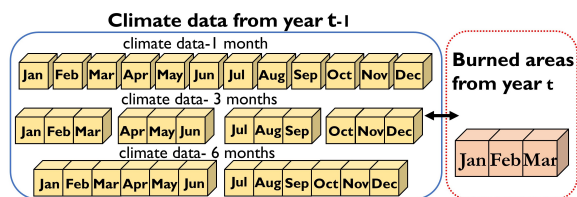
Figure 5: Data modeling approach: For each cell in each landscape, climate data from previous year t-1 and other static features are used as covariates corresponding to the binary observations of burned areas during the fire season in the current year t . This data point generation scheme holds for all locations N and all years T in \mathcal{D} .
