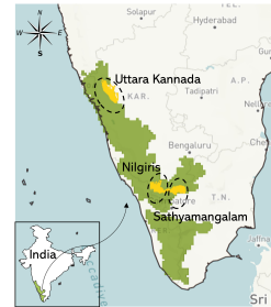
Figure 1: Southern Western Ghats is shown in green and three landscapes studied in this paper are shown in yellow. In total these landscapes cover 5306 sq. km.
