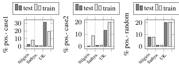
Figure 7: Imbalance across observation labels for different partitioning approaches. Case 1 & 2: temporal division; random: random partitioning with no time consideration.
