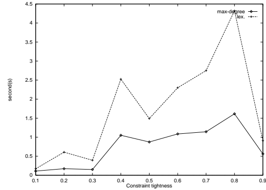
Figure 2. DCSPs with 15 variables, 5 values per domain, and 30% of connectivity (cpu time)
