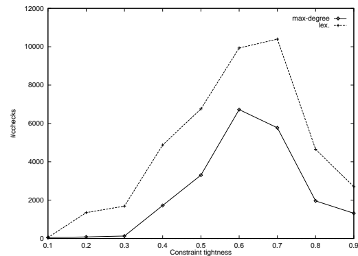
Figure 3. DCSPs with 15 variables, 5 values per domain, and 30% of connectivity (constraint checks)
