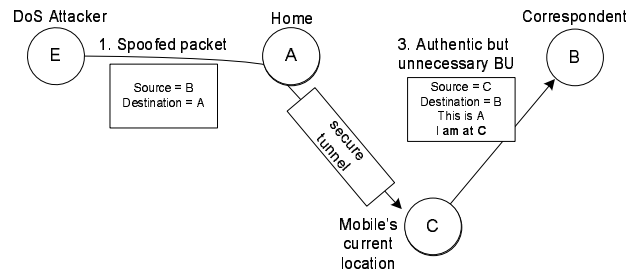
Fig. 6. Inducing unnecessary BUs
