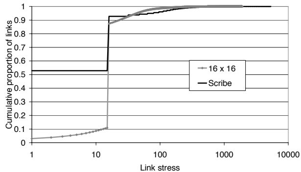
(b) SplitStream vs Scribe
