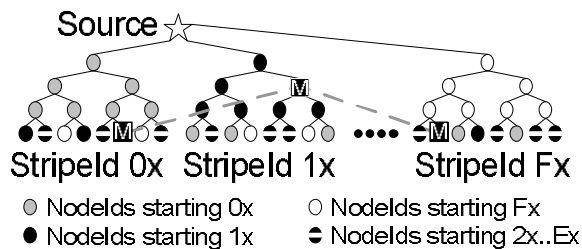
Figure 4: SplitStream’s forest construction. The source splits the content and multicasts each stripe in its designated tree. Each stripe’s stripeId starts with a different digit. The nodeIds of interior nodes share a prefix with the stripeId, thus they must be leaves in the other trees, e.g., node M with a nodeId starting with 1 is an interior node in the tree for the stripeId starting with 1 and a leaf node in other trees.
