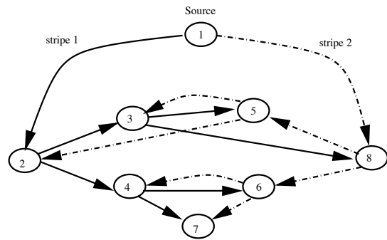
Figure 1: A simple example illustrating the basic approach of SplitStream. The original content is split into two stripes. An independent multicast tree is constructed for each stripe such that a peer is an interior node in one tree and a leaf in the other.
