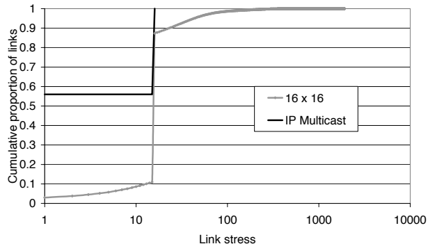
(a) SplitStream vs IP
