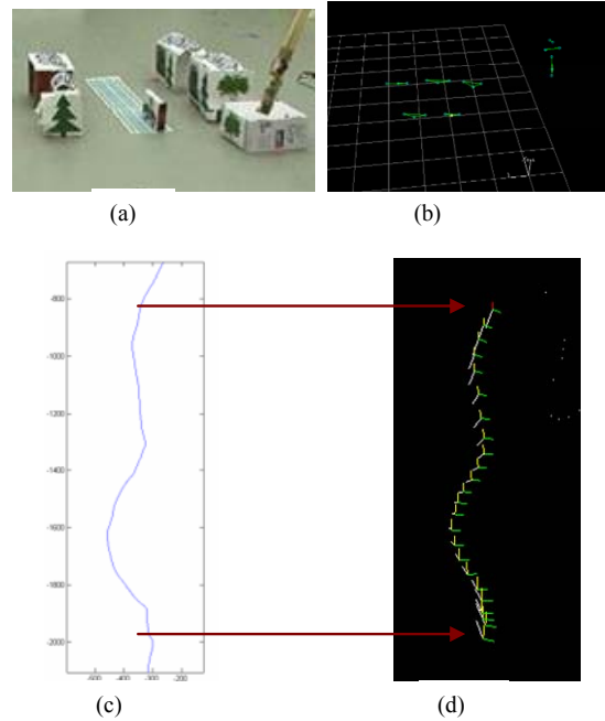
Figure 4.2: Verification by ground truth from motion capture system: (a) the scene model; (b) one view of the motion capture system; (c) camera trajectory from motion capture system; (d) camera trajectory from our vision system.
