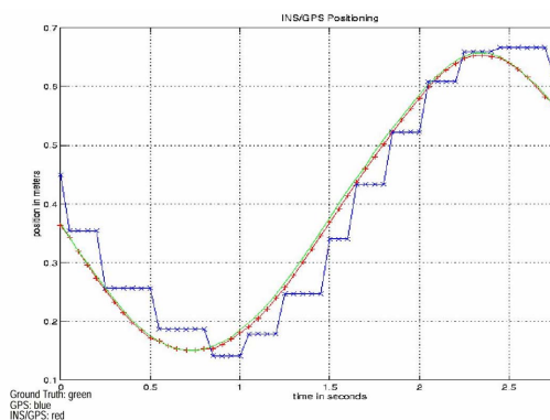
Figure 6 State estimation by GPS/INS integration. The blue line is the GPS position measurement. The red curve is the integrated state estimate while the green curve is the ground truth.
