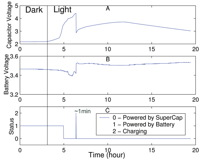
Fig. 10. Telos charges lithium battery from supercapacitors
