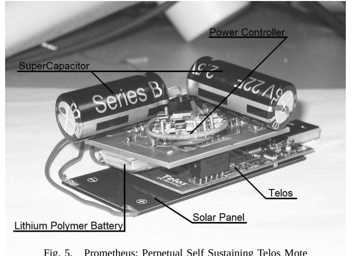
Fig. 5. Prometheus: Perpetual Self Sustaining Telos Mote
