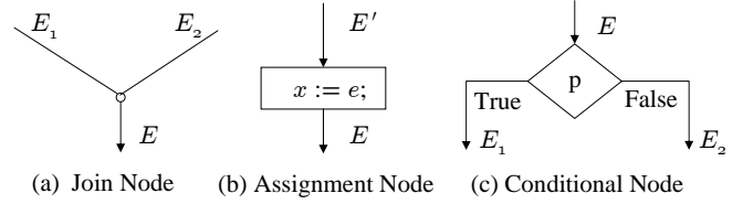
Figure 5. Flowchart Nodes.
