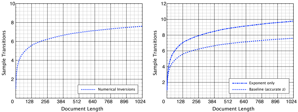
Figure 1: Number of Numerical Inversions and Approximate z Schemes
