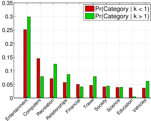
(a) Pr(Category | k < 1) vs. Pr(Category | k > 1)
