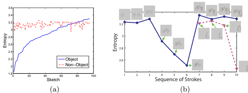
Fig. 4. The entropy of sketches. (a) The entropy comparison between 100 object/non-object pairs. (b) The entropy curve of all steps when drawing a bicycle and a tree. The entropies of the tree with different strokes are also illustrated.
