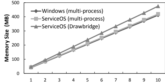
Figure 7: Memory committed for increasing instances of Wordpad. Each new instance loads a 10MB document.
