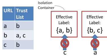
Figure 3: Non-transitivity in Trust. Although the trust lists show that a and b are mutually trusting and b and c are mutually trusting, transitive trust does not follow: a and c do not trust each other (as desired by their trust list specification) and will never share an isolation container.
