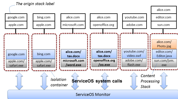
Figure 2: The origin stack as the principal label.
