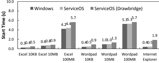
Figure 5: Time to start applications.
