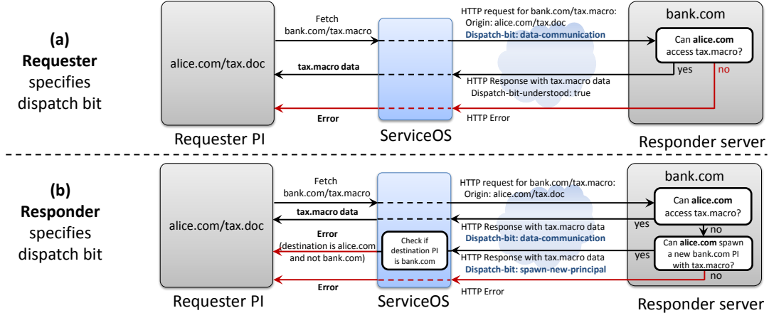
Figure 4: Two design choices for specifying the dispatch bit. Here, a Word application rendering a document from alice.com attempts to retrieve a helper macro from bank.com, to be used in the alice.com principal instance.
