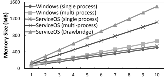
Figure 6: Memory committed for increasing instances of Excel. Each new instance loads a 10MB document.
