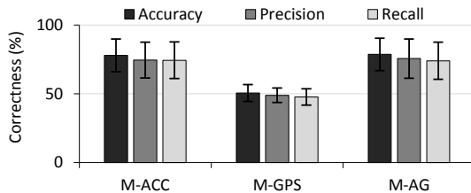
Figure 8: Accuracy for multi-class activity detection.
