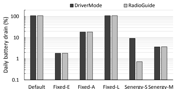
Figure 10: DriverMode and RadioGuide energy with Driving Data.
