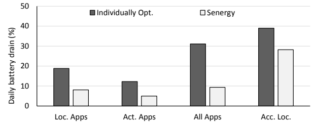
Figure 12: Energy savings when individually optimizing each application and using Senergy. Each case meets the same latency and accuracy requirements. The geometric mean saving is 50.61% compared to individual optimization.
