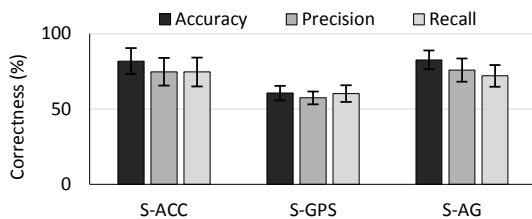
Figure 7: Accuracy for stationary activity.
