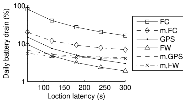
Figure 1: Location Tracking. Latency-energy tradeoffs for six algorithms averaged over four devices. The GPS algorithm only uses GPS data, FC uses network Fingerprints over a Cellular data connection, and FW uses Fingerprints over a WiFi connection. The m,* versions sense location only if they first detect movement using accelerometer data.
