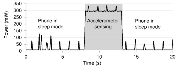
Figure 4: Background accelerometer power
