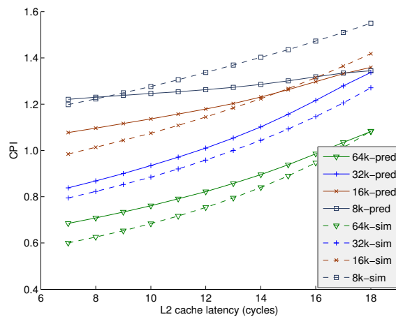
Figure 6. Using RBF network for predicting variation in performance for the vortex benchmark due to different icache sizes and L2 latencies
