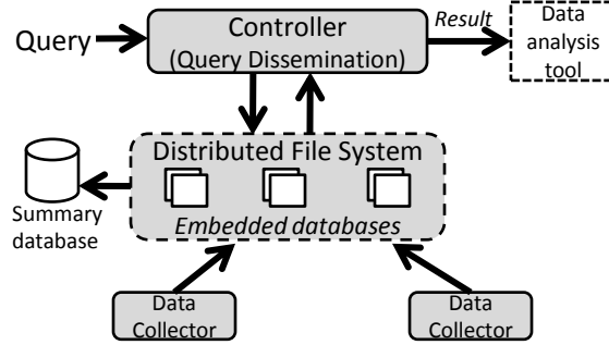
Figure 3: DataGarage Architecture
