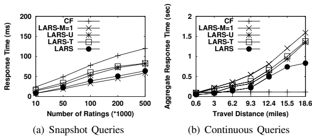
Fig. 10. Query Processing Performance.
