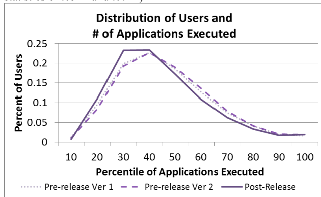
Figure 5: Distribution differences for applications executed
