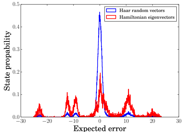
FIG. 7. This plot shows the distribution of expectation values of the error operator for water in the local basis over its eigenstates and Haar random vectors. We see that the random vectors lead to substantially less error, on average, than do the Hamiltonian eigenstates. The Haar distribution of errors has a standard deviation of 4.82 while the Hamiltonian error distribution has standard deviation of 10.68.
