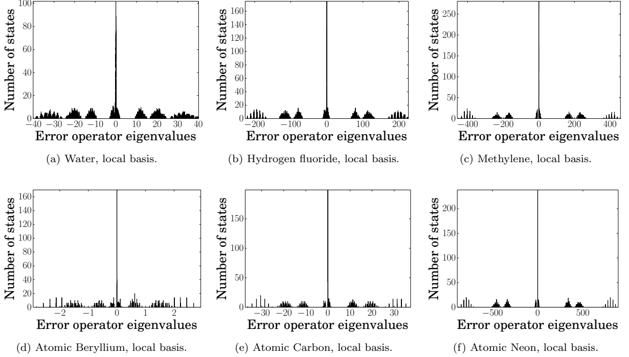
FIG. 8. These are histograms of the eigenspectra of the error operators for various molecular and atomic benchmarks in the local basis. Error operators for all of our benchmarks have surprisingly similar eigenspectra, regardless of the orbital basis. The source of this striking similarity and the reason for the particular structure is unknown.
