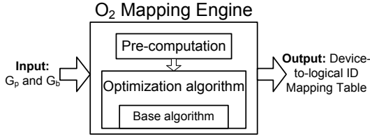
Figure 3: The O_2 mapping engine.
