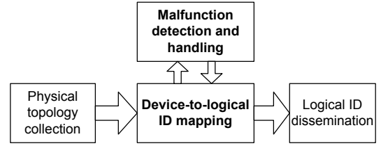
Figure 2: The DAC system framework with four modules.
