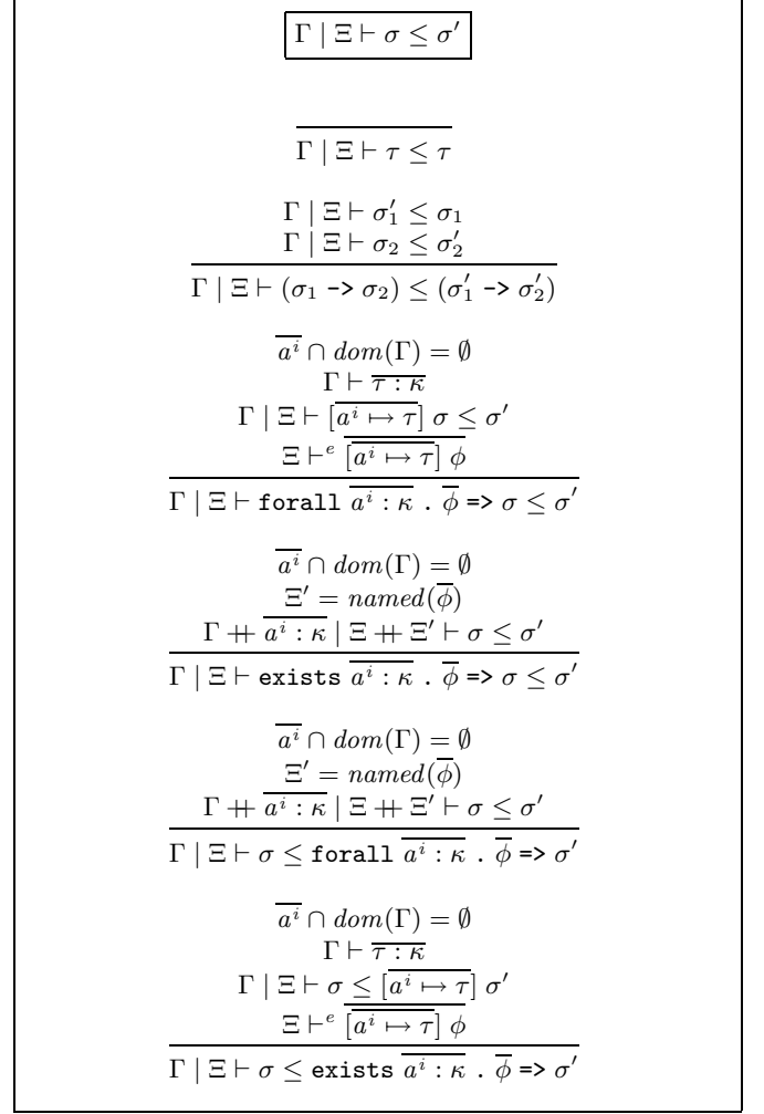
Figure 11: Type subsumption
