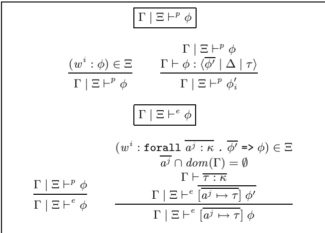
Figure 10: Constraint entailment
