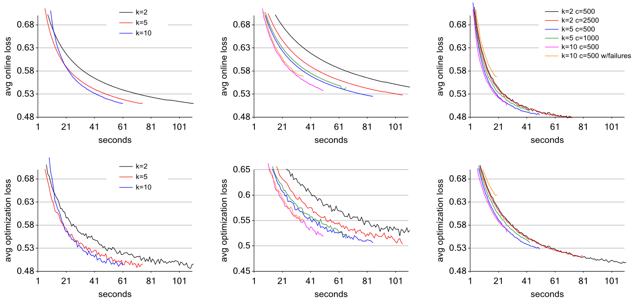
Figure 1. Top: average online loss for DMB (left), MaWo-DMB (center), ADMB(right). Bottom: test loss (on a held-out set) for DMB (left), MaWo-DMB (center), ADMB(right). The mini-batch size in all experiments is b = 5000 . In each plot, k denotes number of nodes and c denotes chunk size.
