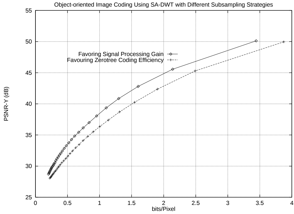
Figure 11: Comparison of different subsampling strategies in shape adaptive wavelet coding (Akiyo-CIF).
