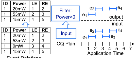
Fig. 2. Events, CQ plans, lifetimes.
