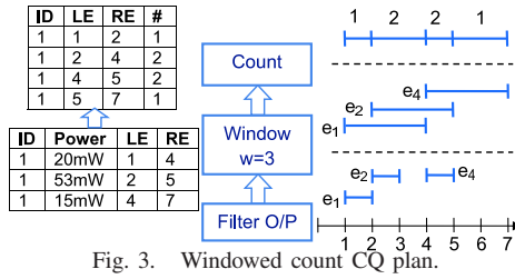
Fig. 3. Windowed count CQ plan.
