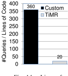
Fig. 14. Lines of code & processing time.
