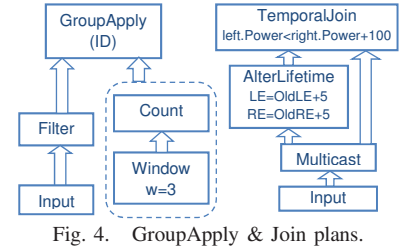
Fig. 4. GroupApply & Join plans.
