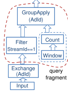
Fig. 7. Annotated CQ plan for RunningClickCount.
