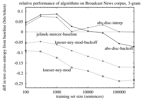
Figure 16: Performance relative to baseline of backoff and interpolated versions of absolute discounting and modified Kneser-Ney smoothing on Broadcast News corpus, bigram and trigram models
