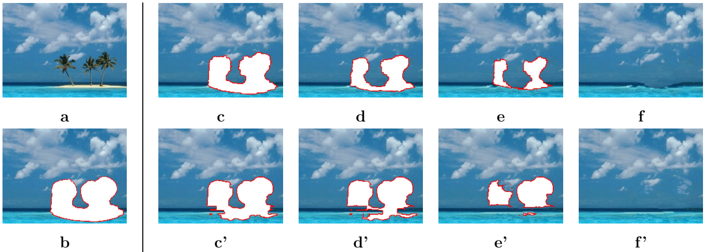
Figure 19: Concentric-layer filling vs. the proposed guided filling algorithm. (a) Original image. (b) The manually selected target region (20% of the total image area) has been marked in white with a red boundary. (c,d,e,f) Intermediate stages in the concentric-layer filling. The deformation of the horizon is caused by the fact that in the concentric-layer filling sky and sea grow inwards at uniform speed. Thus, the reconstructed sky-sea boundary tends to follow the skeleton of the selected target region. (c',d',e',f') Intermediate stages in the filling by the proposed algorithm, where the horizon is correctly reconstructed as a straight line.
