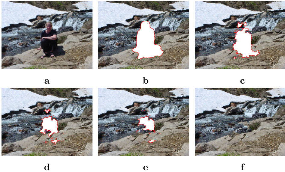
Figure 20: Removing large objects from photographs. (a) Original image. (b) The target region (10% of the total image area) has been blanked out. (c...e) Intermediate stages of the filling process. (f) The target region has been completely filled and the selected object removed. The source region has been automatically selected as a band around the target region. The edges of the stones have been nicely propagated inside the target region together with the water texture.
