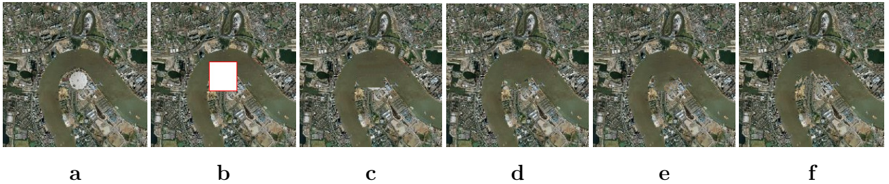
Figure 9: Effect of filling order on an aerial photograph. (a) The original image, an aerial view of London. (b) The target region has been selected and marked with a red boundary; Notice that it straddles two different textures; (c) Filling with raster-scan order; (d) Filling by concentric layers; (e) The result of applying Harrison's technique (performed in 45"); (f) Filling with our algorithm (performed in 2"). See text for details.
