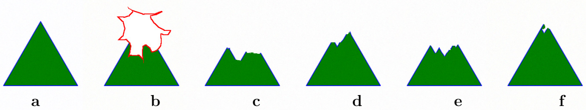
Figure 8: Effect of filling order on a synthetic image. (a) The original image; (b) The target region has been selected and marked with a red boundary; (c) Filling the target region in raster-scan order; (d) Filling by concentric layers; (e) The result of applying Harrison's technique which took 2' 45"; (f) Filling with our algorithm which took 5". Notice that even though the triangle upper vertex is not complete our technique performs better than the others.
