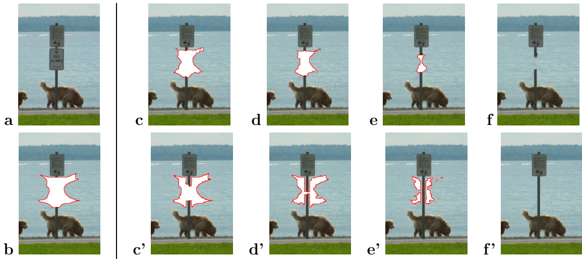
Figure 11: Onion peel vs. structure-guided filling. (a) Original image. (b) The target region has been selected and marked with a red boundary. (c,d,e,f) Results of filling by concentric layers. (c’,d’,e’,f’) Results of filling with our algorithm. Thanks to the data term in (1) the sign pole is reconstructed correctly by our algorithm.
