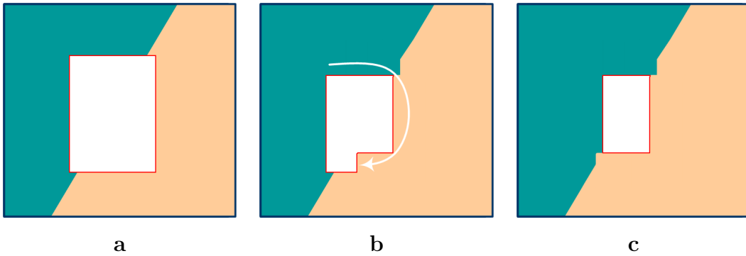
Figure 4: The importance of the filling order in patch-based filling. (a) The target region is shown in white. (b) Part of the outmost layer in the target region has been synthesized by an onion-peel algorithm proceeding in clock-wise order. (c) At a further stage of the filling process, the remainder of the outmost layer has been filled by this clock-wise onion-peel filling. The concentric-layer filling has produced artefacts in the reconstruction of the diagonal image edge. A filling algorithm whose priority is guided by the image edges would fix this problem.
