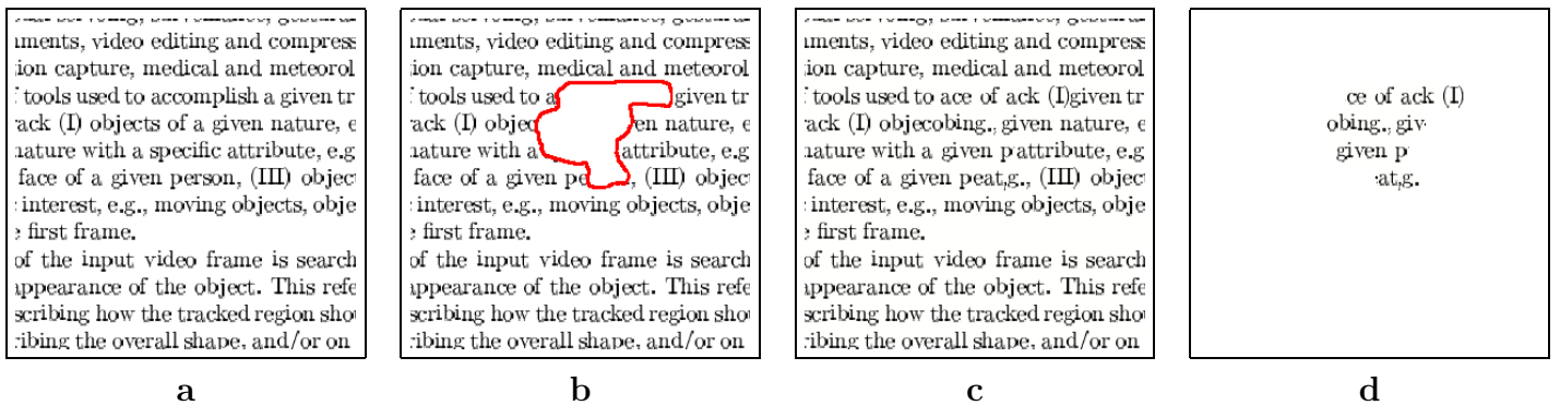
Figure 22: Region-filling on an image of a text. (a) Original photo of typewritten text, a favourite example of texture synthesis researchers. (b) A portion of the image (marked with a red boundary) has been removed. (c) The result of our filling algorithm. (d) As in (c) with just the text synthesized in the target region highlighted. Even though the generated text does not make much sense it still looks plausible. This example further demonstrates the correct behaviour of our algorithm in the case of pure texture synthesis.
