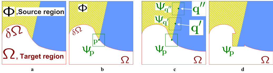
Figure 2: Structure propagation by exemplar-based texture synthesis. (a) Original image, with the target region \Omega , its contour \delta\Omega , and the source region \Phi clearly marked. (b) We want to synthesize the area delimited by the patch \Psi_{\mathbf{p}} centred on the point \mathbf{p} \in \delta\Omega . (c) The most likely candidate matches for \Psi_{\mathbf{p}} lie along the boundary between the two textures in the source region, e.g., \Psi_{\mathbf{q}'} and \Psi_{\mathbf{q}''} . (d) The best matching patch in the candidates set has been copied into the position occupied by \Psi_{\mathbf{p}} , thus achieving partial filling of \Omega . Notice that both texture and structure (the separating line) have been propagated inside the target region. The target region \Omega has, now, shrunk and its front \delta\Omega has assumed a different shape.
