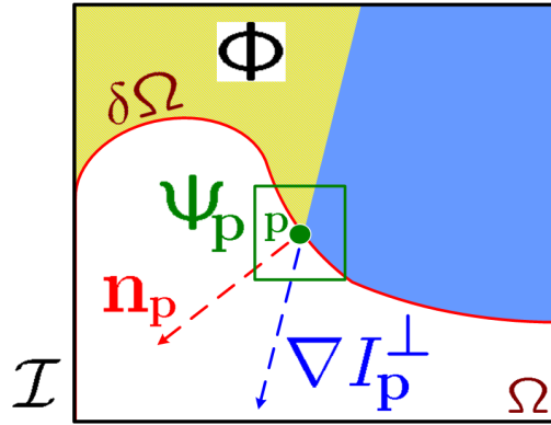
Figure 5: Notation diagram. Given the patch \Psi_{\mathbf{p}} , \mathbf{n}_{\mathbf{p}} is the normal to the contour \delta\Omega of the target region \Omega and \nabla I_{\mathbf{p}}^{\perp} is the isophote (direction and intensity) at point \mathbf{p} . The entire image is denoted with \mathcal{I} .
