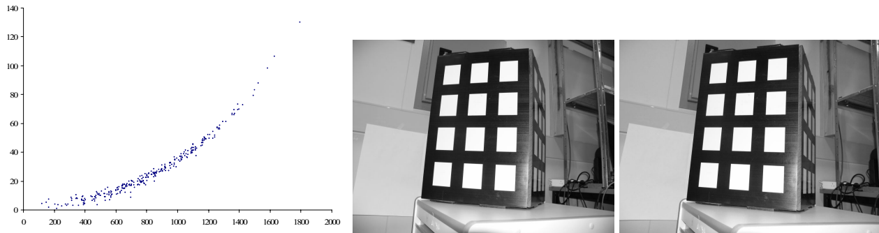
Figure 11: Results for the non-planar calibration experiment. From left to right: extracted distortion graph, original image, and corrected images.
