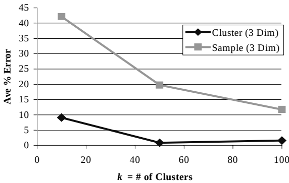
Figure 7: Varying k on Investor dataset.
