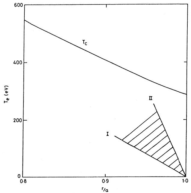
FIG. 6. Graph of Fig. 4 converted to a T_c(r) curve. Also shown are the first and second marginally stable temperature gradients for r = a , T = 0 .
