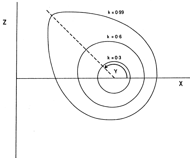
FIG. 1. Example of flux surfaces used in construction of model equilibrium.
