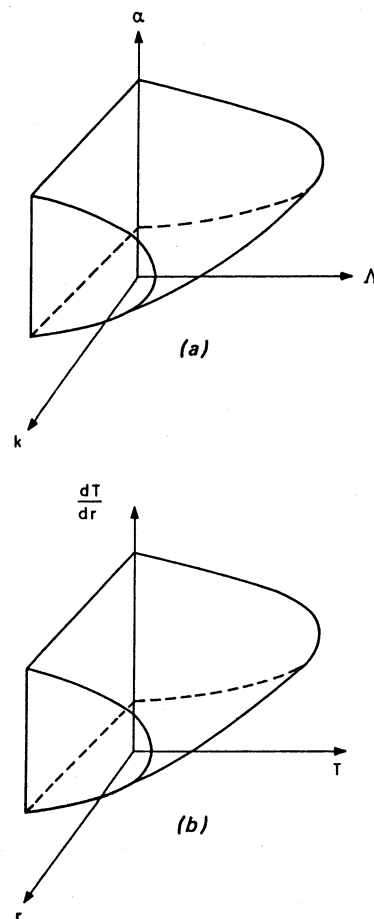
FIG. 5. (a) Ballooning unstable zone shown schematically in (\alpha, \Lambda, k) space. (b) Stability diagram corresponding to (a) but plotted in (dT/dr, T, r) space.
