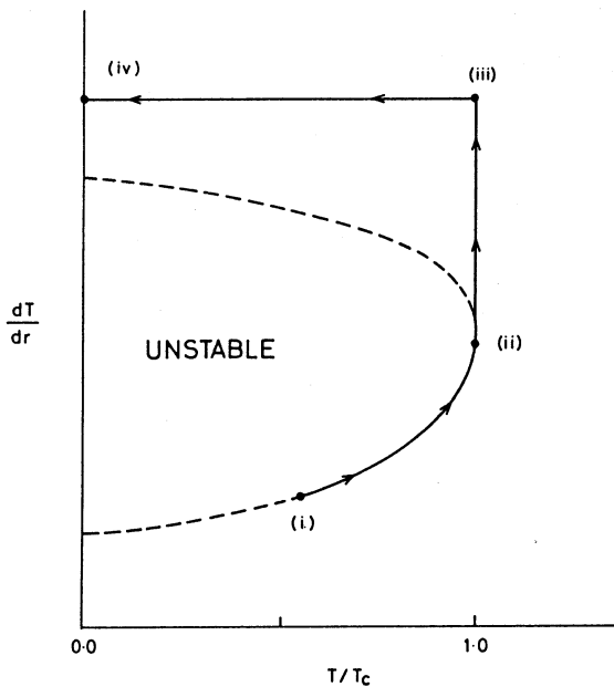
FIG. 8. Ballooning unstable zone projected onto (dT/dr, T/T_c) plane, showing the trajectory of a class II profile.
