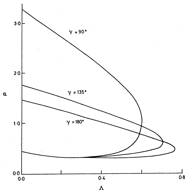
FIG. 9. Dependence of stability boundaries, and \Lambda_c , on the X-point location \gamma ( k = 0.95 ).
