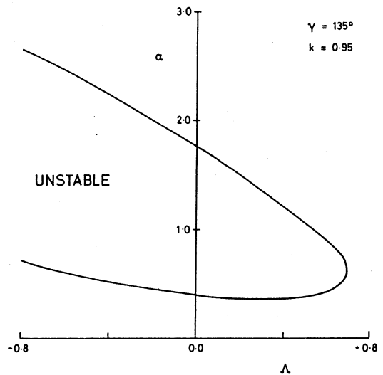
FIG. 2. Unstable zone in \alpha - \Lambda plane showing the existence of a critical value of \Lambda ( \gamma = 135^\circ ).
