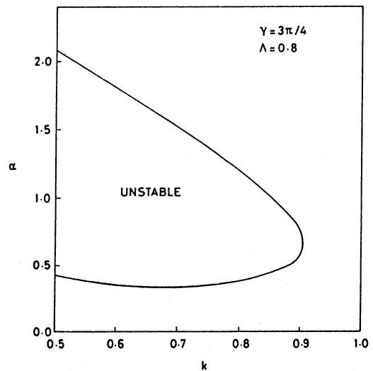
FIG. 3. Stability diagram in the \alpha - k plane at \Lambda = 0.8 ( \gamma = 135^\circ ).
