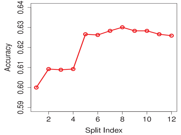
Figure 3: Classification accuracy of the CR algorithm on mobile video chat data using different split thresholds.
