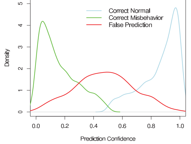
Figure 6: Bidirectional confidence distribution generated by Weka for binary classification.
