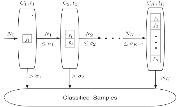
Figure 5: K -stage cascaded classifier.
