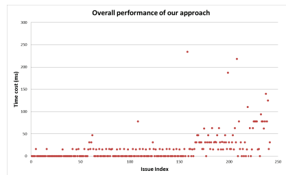
Figure 6. Overall performance of our approach
