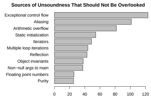
Figure 4: Ranking of the sources of unsoundness in program analysis that developers indicated should not be overlooked (i.e., considering them during analysis would be most helpful to developers).
