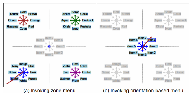
Figure 10. Hybrid Zone-Orientation menu of breadth-40. (a) If the first stroke is a short tap, it invokes the Zone menu. (b) A longer first stroke invokes the orientation-based menu.
