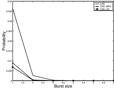
Fig. 3. Probability vs Burst Size, offered load = 0.85, for CAC, CAC-MPC and CAC-UC
