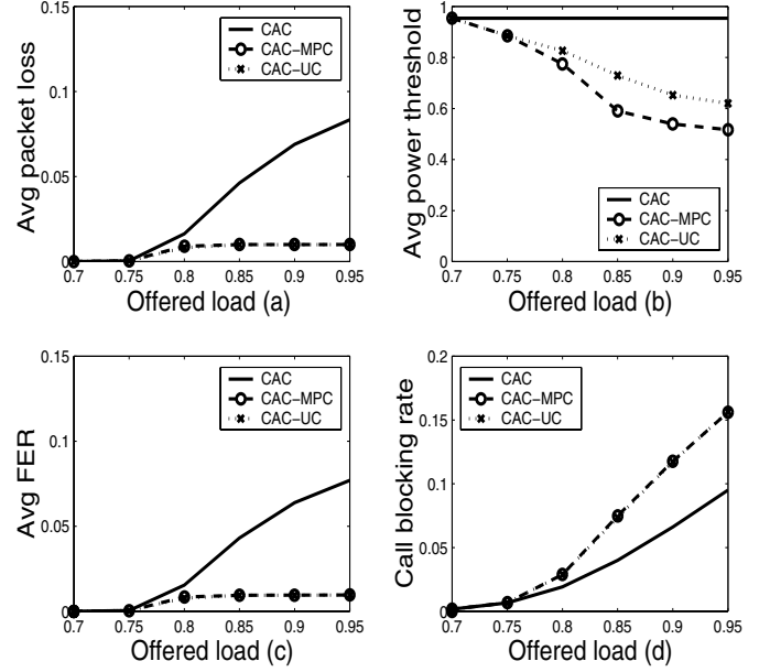
Fig. 2. Performance metrics of CAC, CAC-MPC, and CAC-UC as a function of offered load: (a) average packet loss rate; (b) average power threshold; (c) average frame error rate; (d) average call blocking rate.
