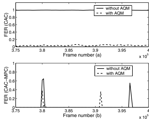
Fig. 9. FER vs Frame Number, Offered Load = 85%, Maximum Router Queuing Delay = 30ms (a) CAC (b) CAC-MPC
