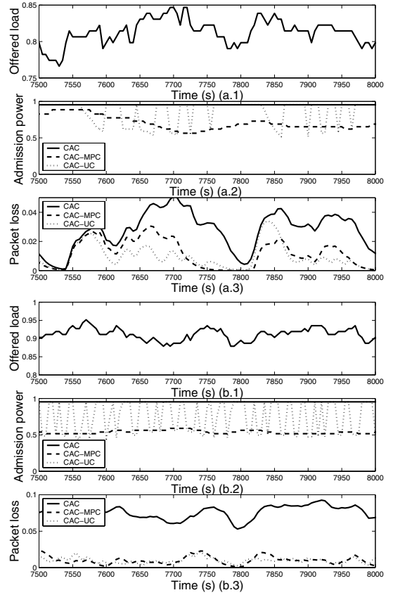
Fig. 4. Time variation of offered load, power threshold and packet loss rate for CAC, CAC-MPC and CAC-UC: (a) at offered load 0.8; (b) at offered load 0.9
