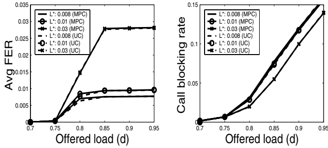
Fig. 6. Performance metrics of CAC, CAC-MPC, and CAC-UC as a function of offered load at target loss rate 0.008, 0.01, and 0.03: (a) average frame error rate; (b) average call blocking rate.
