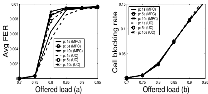
Fig. 7. Performance metrics of CAC, CAC-MPC, and CAC-UC as a function of offered load with control interval 1s, 5s, and 10s: (a) average frame error rate; (b) average call blocking rate.
