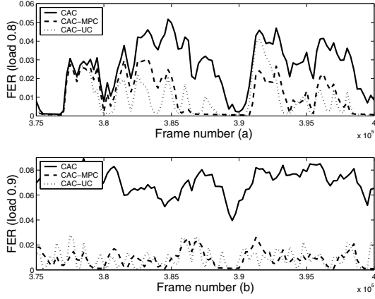
Fig. 5. Time variation of the received voice frame error rate: (a) at offered load 0.8; (b) at offered load 0.9.
