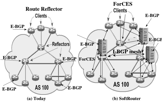
Figure 3: BGP deployment
