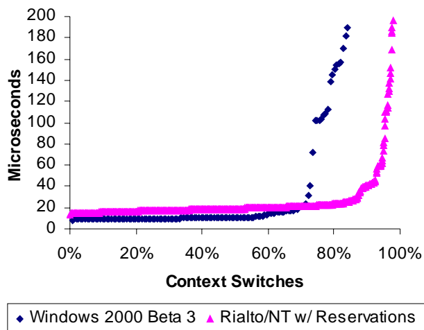
Figure 4-1: Rialto/NT vs. native context switch times
