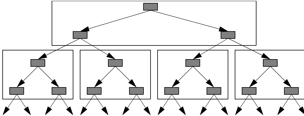
Figure 1. Subtree clustering.
