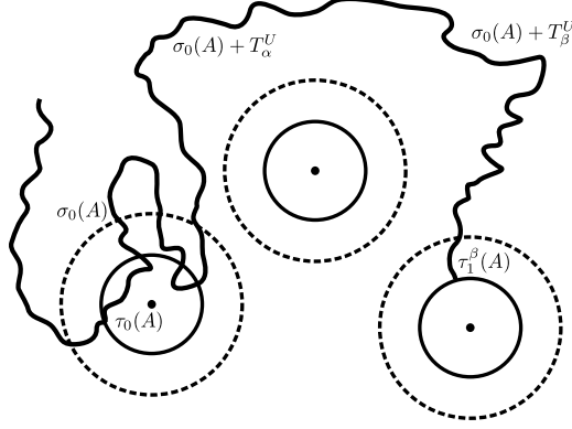
FIG. 3. The solid and dashed circles represent the boundaries of A(r) and A(R) , respectively, and the small points are the elements of A . Note that X may re-enter A(r) during the interval [\sigma_k^\beta(A), \tau_{k+1}^\beta(A)] .
