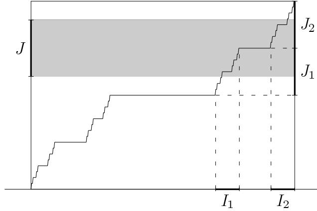
FIGURE 4. An interval J \subset [0, 1] can be covered by two dyadic intervals J_1 and J_2 of comparable size. Intervals I_1, I_2 \in \mathfrak{C}_{\gamma, n} are such that f_\gamma(I_i) = J_i , for i = 1, 2 .
