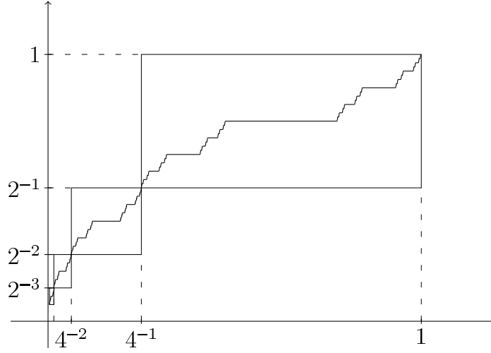
FIGURE 5. Construction of the function f from Remark 3.2. On each interval [4^{-n-1}, 4^{-n}] function f is a scaled and shifted copy of the Cantor function (on the interval (1, \infty) the function is defined arbitrarily).
