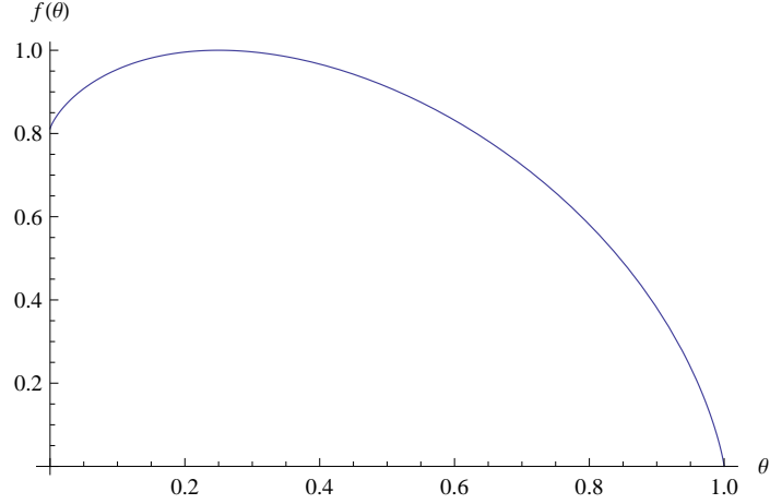
FIGURE 1. Dimension of A_\theta
