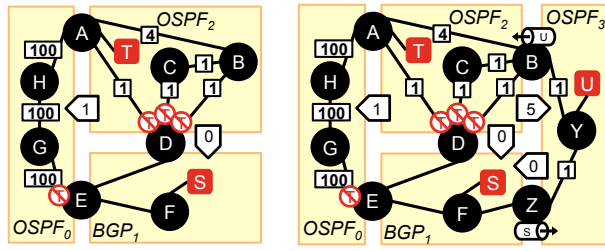
(a) Initial control plane
