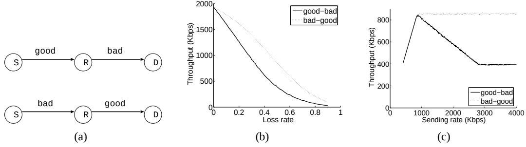
Figure 1: The importance of rate feedback. (a) Two topologies that differ in where the lossy link occurs. (b) Throughput as a function of loss rate when S sends as fast as possible. (c) Throughput as a function of the sending rate when the loss rate of the bad link is 0.50.
