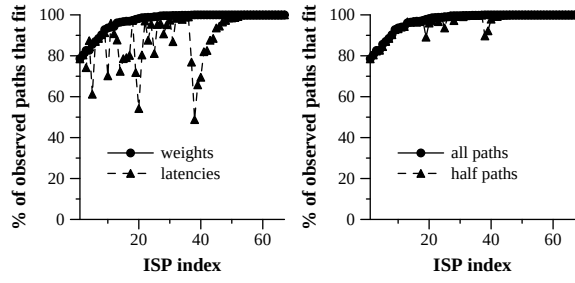
Figure 4: The success of the inferred weights in describing the observed routing. Each point along the x-axis corresponds to an ISP. The y-axis values depict the percentage of observed paths that were least cost. The left graph compares weights with latencies, and the right graph compares the weights inferred using the complete dataset with those inferred using half of it.
