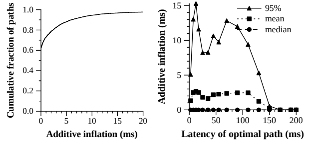
Figure 13: The path inflation due to early-exit compared to optimal exit.
