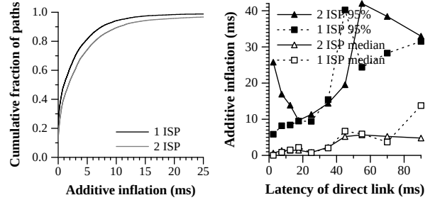
Figure 6: The cost of crossing an ISP boundary compared to intra-domain paths. The left graph shows the CDF of additive inflation over a hypothetical direct link between the city pair for paths that cross an ISP boundary (2 ISP) and intra-domain paths (1 ISP). The right graph shows the variation of median and 95th percentile inflation with the baseline hypothetical distance between the city pair.
