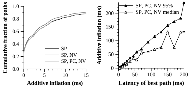
Figure 16: Path inflation due to common AS policies. With the latency of the lowest-latency path as a reference (the x -axis), we show the inflation when choosing shortest AS paths (SP), then choosing only valley-free paths (NV), then additionally preferring customer (PC) routes. At right, only the no-valley, prefer-customer inflation is shown; the other lines are similar.
