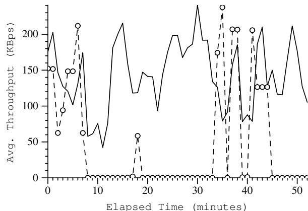
Figure 9: Average throughput of cooperative nodes (solid line) and free-riders (dashed line) as a function of time. Throughput was calculated using one minute intervals. There were three free-riders. The punishment interval is 30 minutes.
