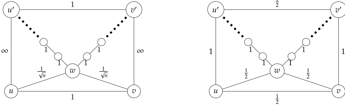
Figure 1. The left diagram represents the \lambda values of the edges, while the right diagram represents the approximate probability of each edge. The example shows that although \mathbb{P}[(u, v) \in T] \approx \frac{1}{2} , and the expected degree of u and v is 2, \mathbb{P}[\deg_T(u) + \deg_T(v) = 3] = 1 - o(1) . Therefore (u, v) is not good. Note that this is not exactly a solution to LP_{\text{subtour}} , but still points to difficulties in proving a trivial edge is good.
