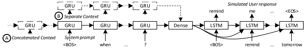
Figure 1: Architecture of seq-2-seq models with encoders (GRU) and decoder (LSTM) unrolled over 'time' (word sequences).
